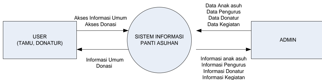
Gambar 2. Context Diagram
