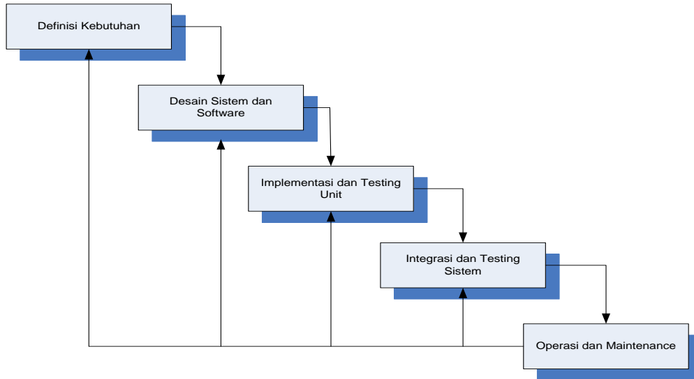
Gambar 1. Model Waterfall Sommerville
