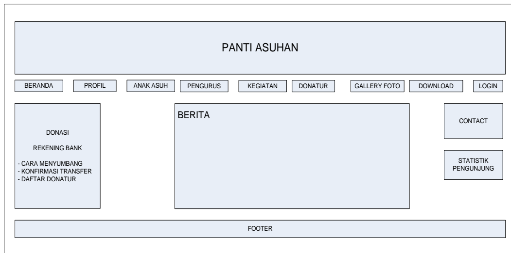
Gambar 3. Rancangan User Interface
